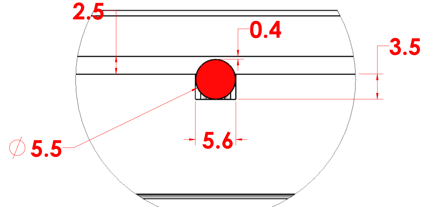
DETAIL B SCALE 4 : 1
