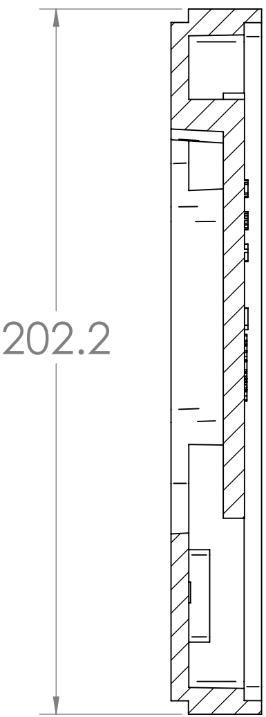
SECTION B-B SCALE 1 : 1.5
