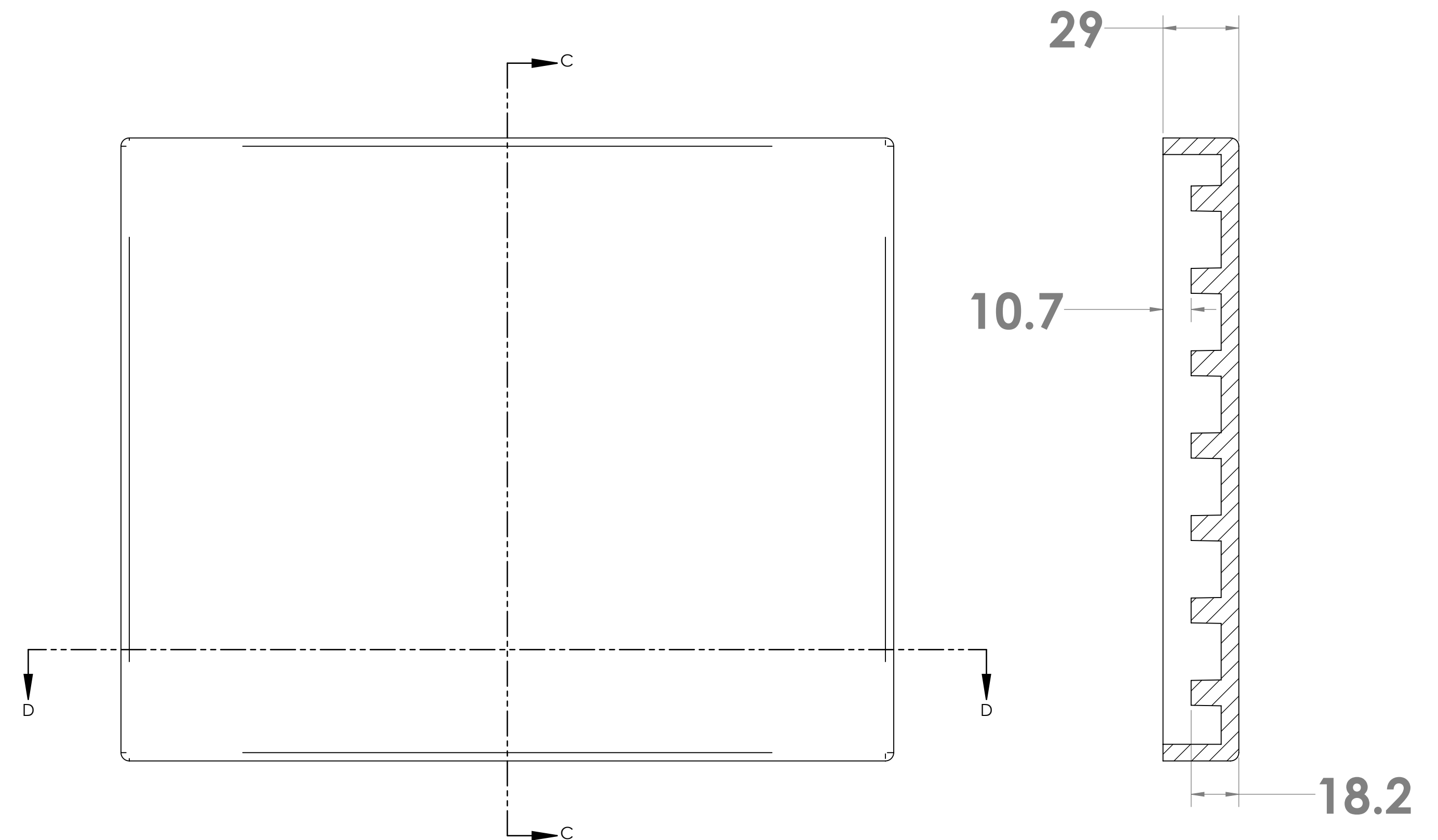
SECTION C-C SCALE 1 : 1.5
