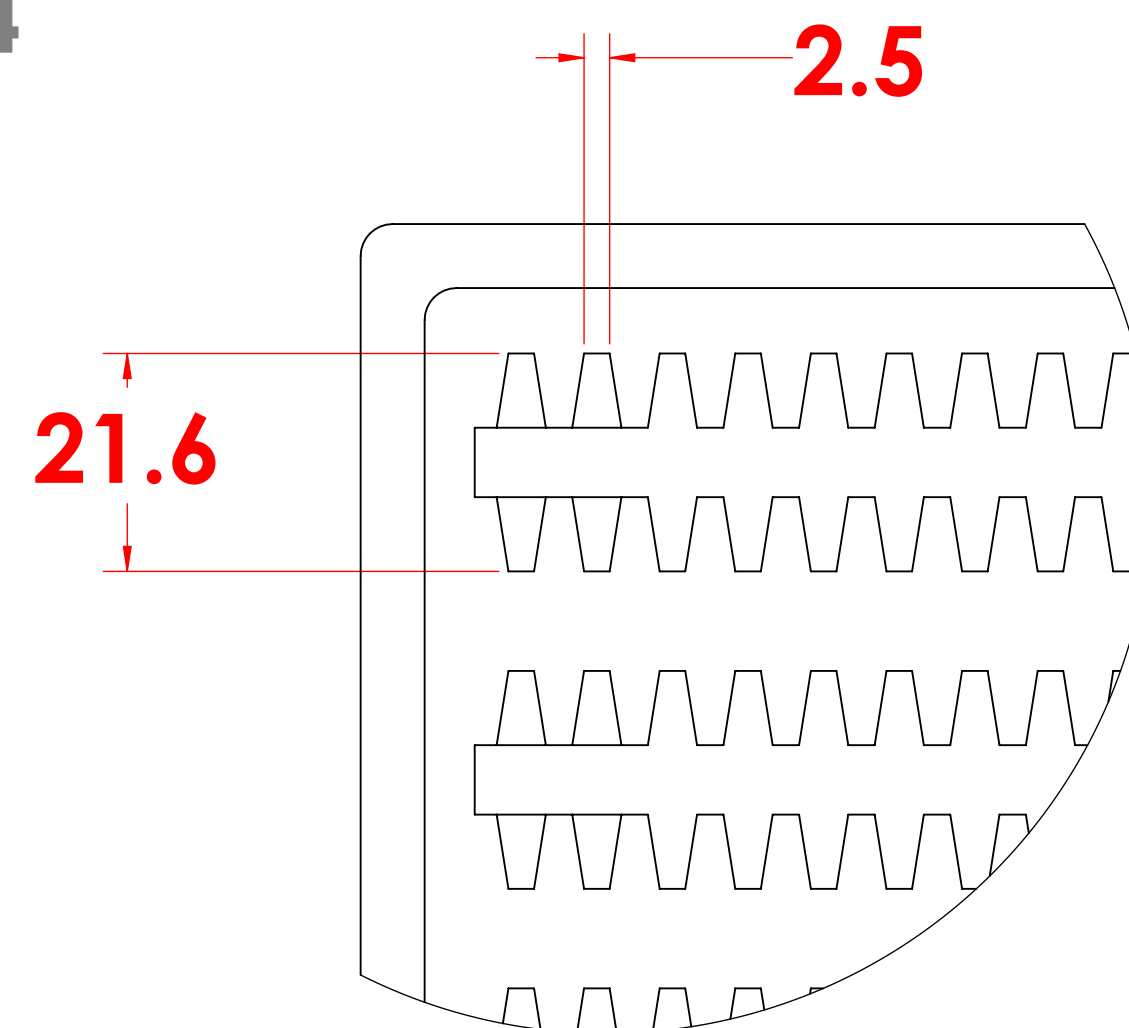
DETAIL E SCALE 2 : 1.5
