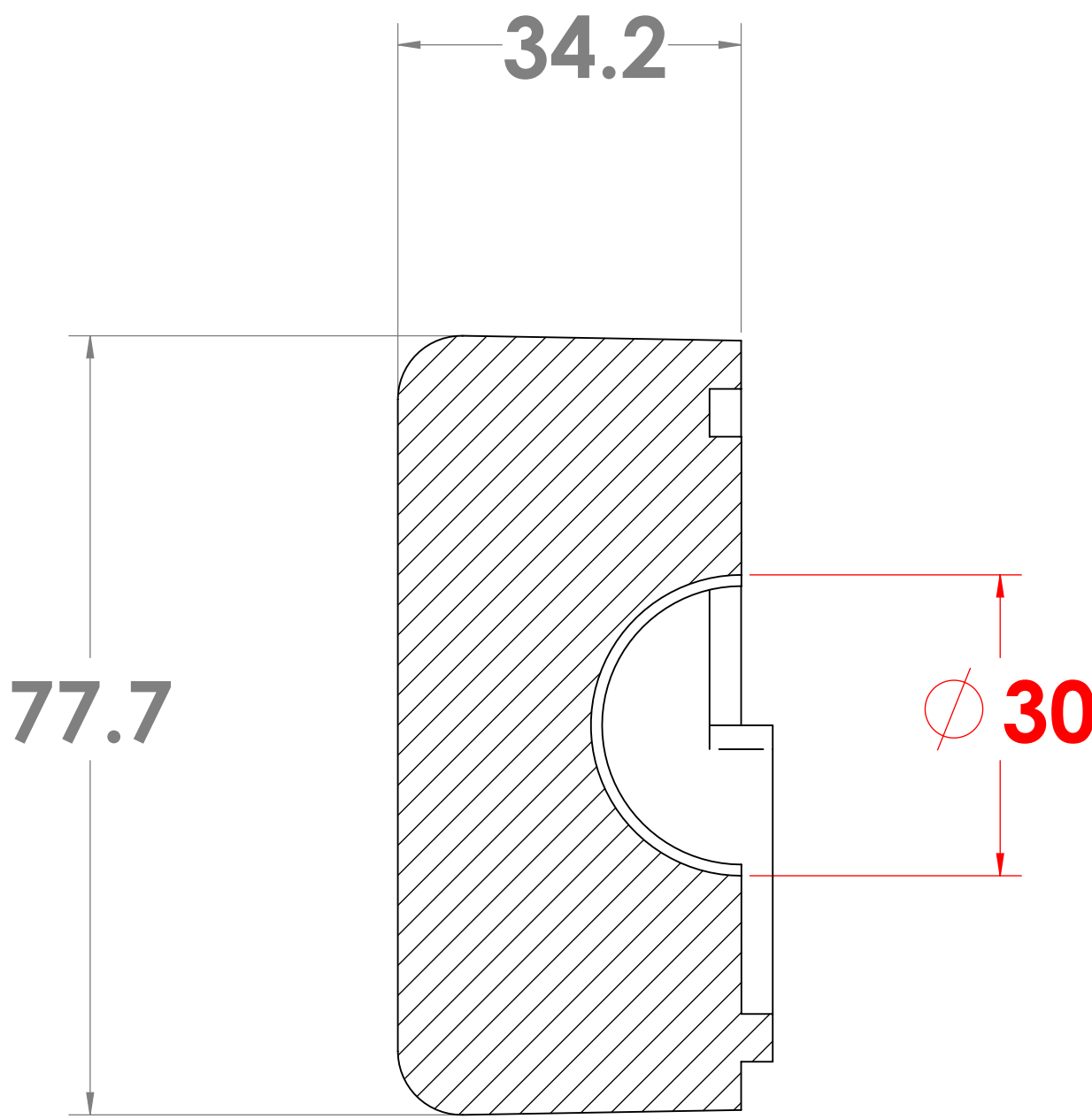
SECTION B-B SCALE 1.5 : 1
