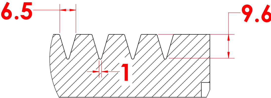
DETAIL C SCALE 2 : 1.5
