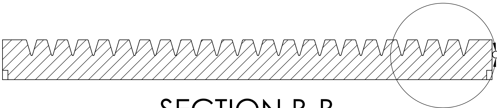
SECTION B-B SCALE 1 : 1.5
