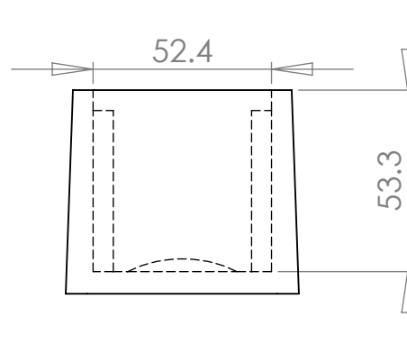
FRONT VIEW OF BASE
