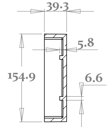
SECTION C-C SCALE 1 : 4
