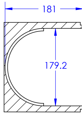
SECTION C-C
