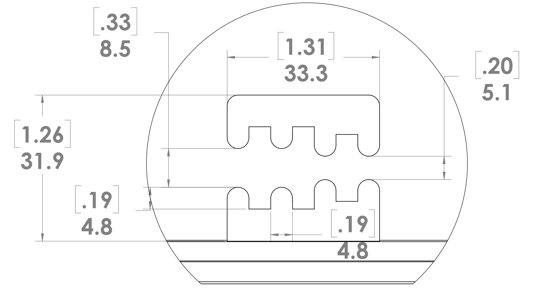
DETAIL B SCALE 2 : 1
