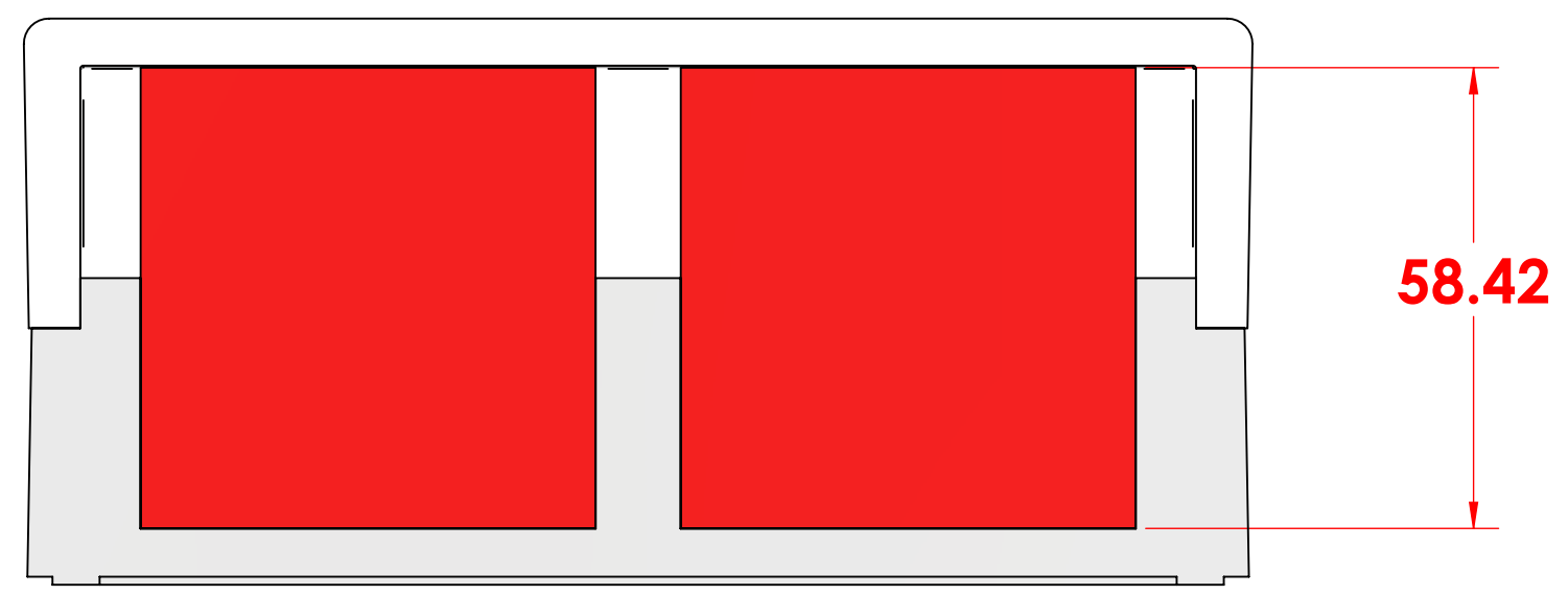
Using #201-01 Lid you can put upto 58.42 x 56.64 x 6.35mm
