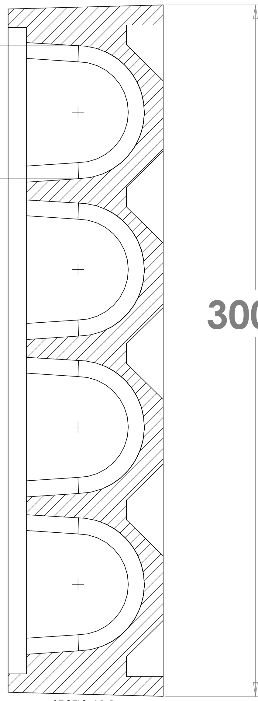
SECTION B-B SCALE 1 : 1
