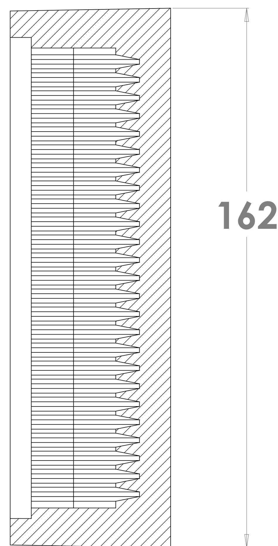
SECTION B-B SCALE 1.5 : 1
